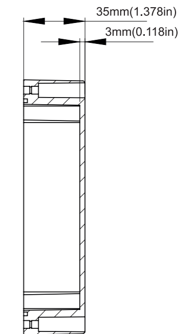
SECTION B-B
