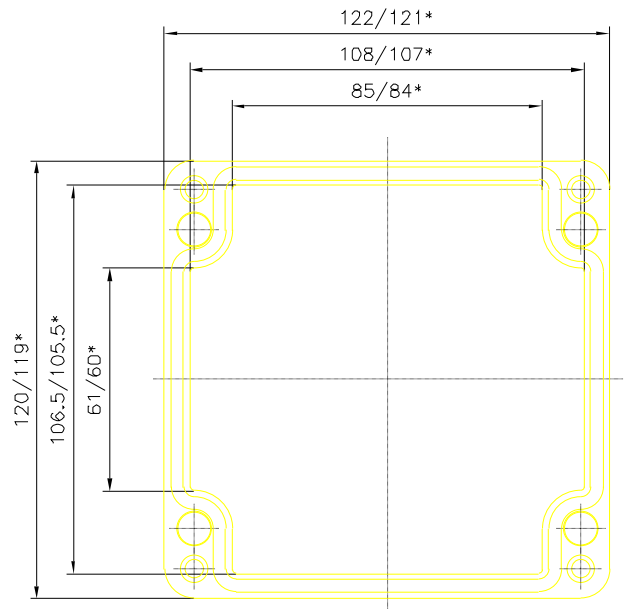
Deckel
