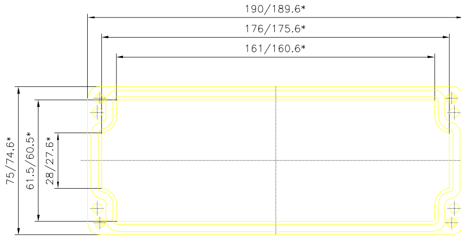
Deckel
