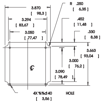
BOTTOM COVER, TOP PCB SCALE 0.650
