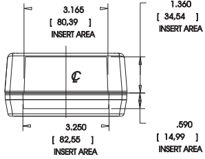
BOTTOM COVER, TOP PCB SCALE 0.650
