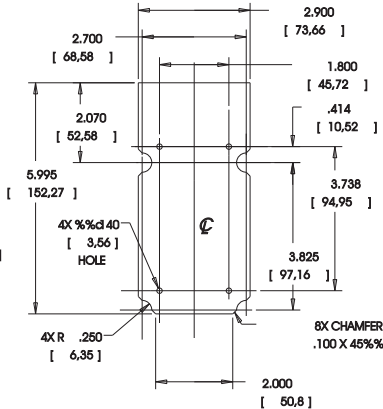
TOP COVER, BOTTOM PCB SCALE 0.650
