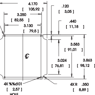
TOP COVER, TOP PCB SCALE 0.650
