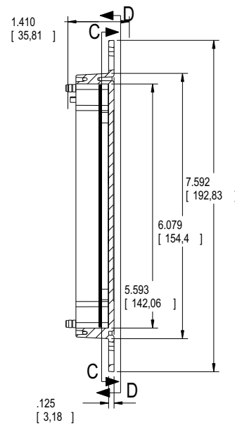
SECTION B-B
