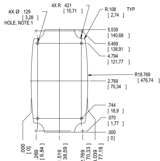
MAX PCB SIZE: .063 TK
